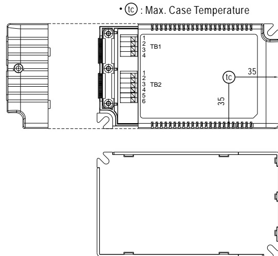
Terminal Pin No. Assignment(TB2)
